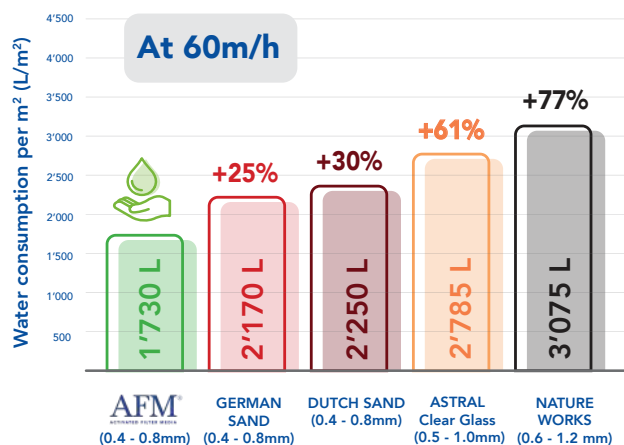
Water consumed per m² of filter surface to backwash filter
